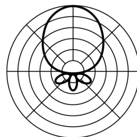
SECOND-ORDER CARDIOID
